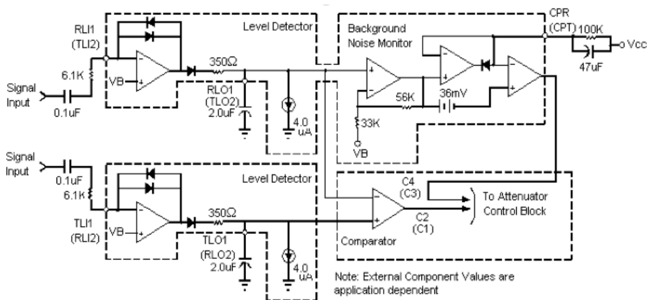
Figure 4. Level Detector
