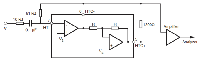
Figure 1. Hybrid Amplifier Distortion Test
