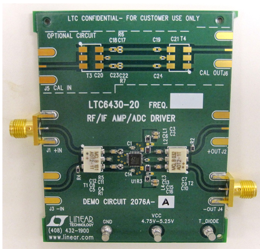
Figure 21. Demo Board 2076A PCB
