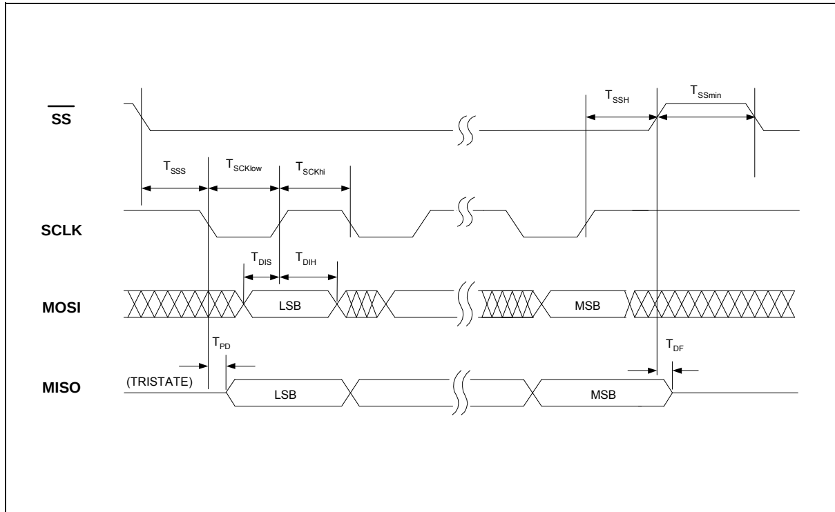
Figure 12.8: SPI Operation
