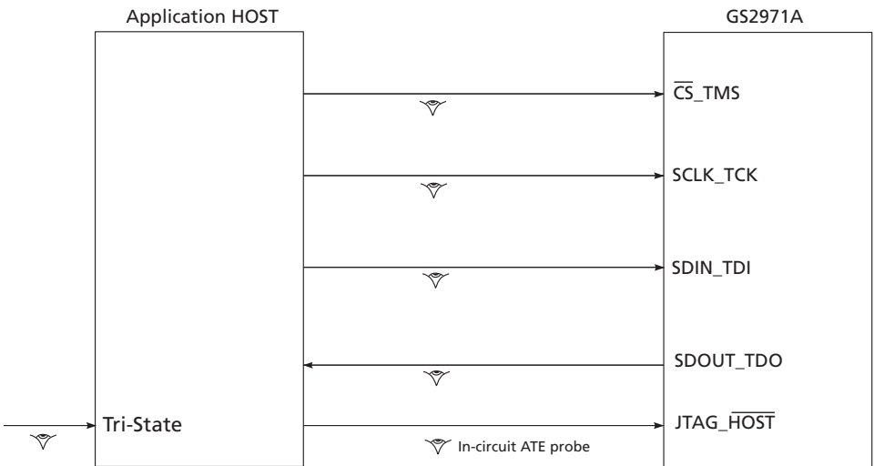
Figure 4-55: System JTAG
