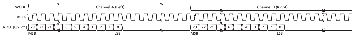
Figure 4-39: Serial Audio, Left Justified, MSB First
