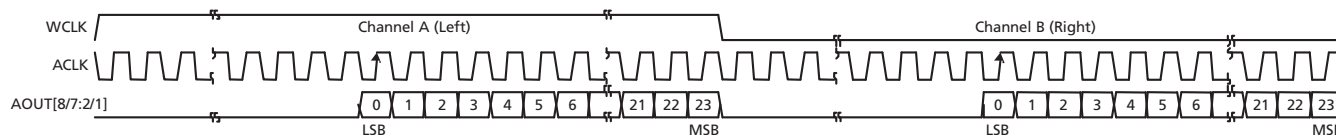
Figure 4-42: Serial Audio, Right Justified, LSB First
