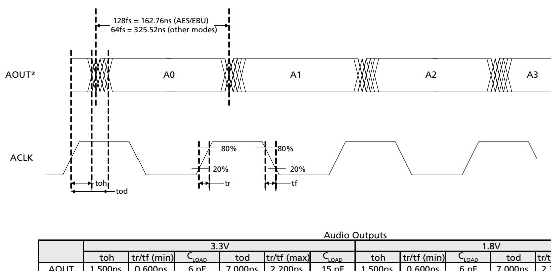
Figure 4-36: ACLK to Data Signal Output Timing
