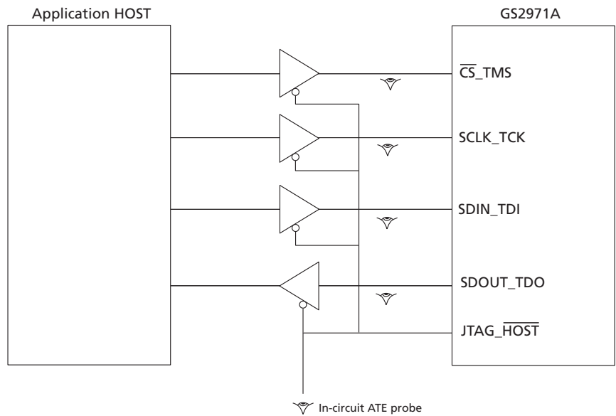
Figure 4-54: In-Circuit JTAG
