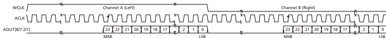
Figure 4-41: Serial Audio, Right Justified, MSB First
