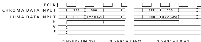
Figure 4-17: H:V:F Output Timing - SD 20-bit Output Mode
