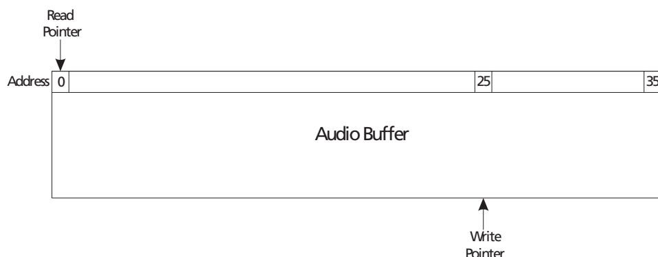
Figure 4-46: Audio Buffer After Initial 26 Sample Write
