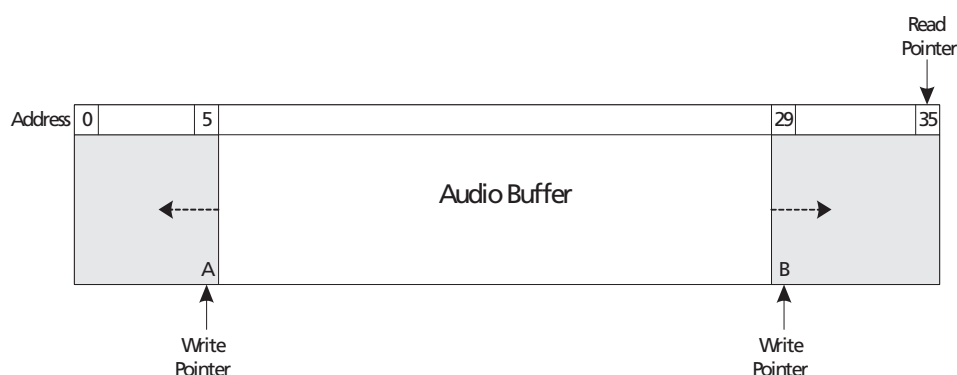
Figure 4-47: Audio Buffer Pointer Boundary Checking
