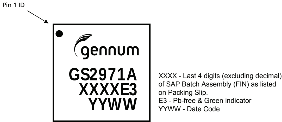
Figure 7-2: GS2971A Marking Diagram
