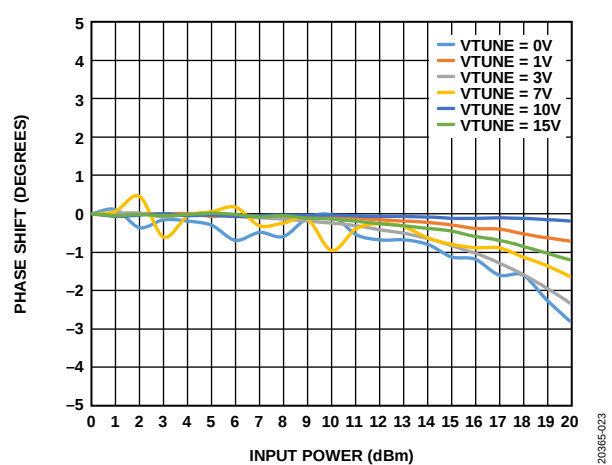
Figure 25. Phase Shift vs. Input Power at Various VTUNE
