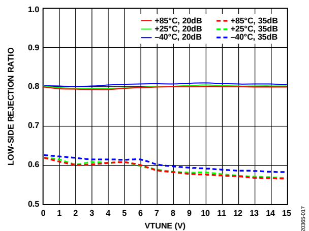
Figure 19. Low-Side Rejection Ratio vs. VTUNE at Various Temperatures and 20 dB and 35 dB
