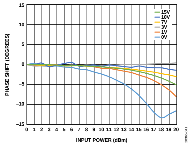
Figure 43. Phase Shift vs. Input Power at Various VTUNE
