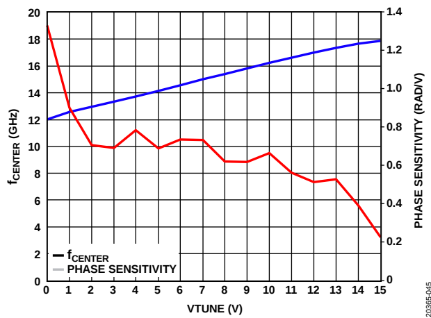
Figure 44. f_{\text{CENTER}} and Phase Sensitivity vs. VTUNE, High Band
