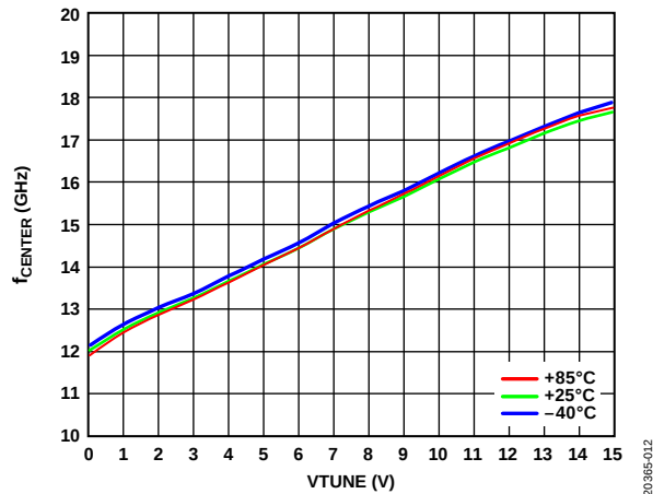
Figure 14. f_{\text{CENTER}} vs. VTUNE at Various Temperatures
