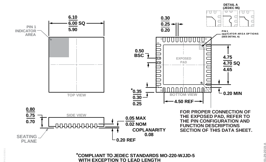
Figure 47. 40-Lead Lead Frame Chip Scale Package [LFCSP] 6 mm × 6 mm Body and 0.75 mm Package Height (CP-40-27) Dimensions shown in millimeters
