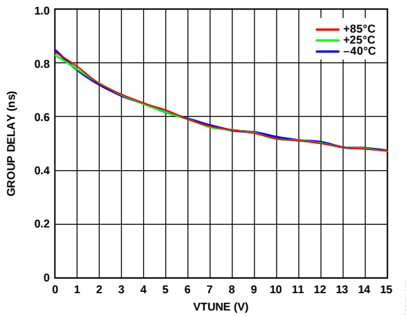
Figure 39. Group Delay vs. VTUNE at Various Temperatures
