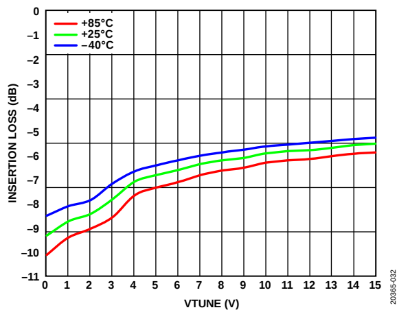
Figure 34. Insertion Loss vs. VTUNE at Various Temperatures
