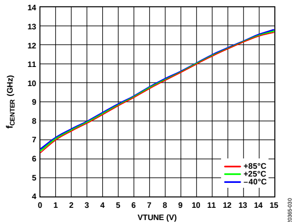
Figure 32. f_{\text{CENTER}} vs. VTUNE at Various Temperatures
