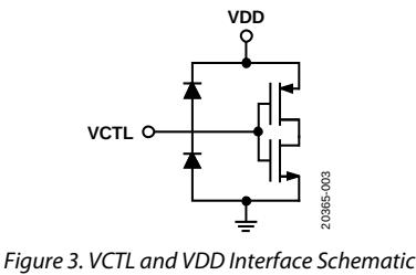
Figure 3. VCTL and VDD Interface Schematic
