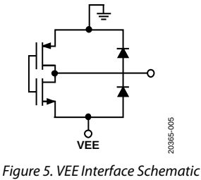
Figure 5. VEE Interface Schematic
