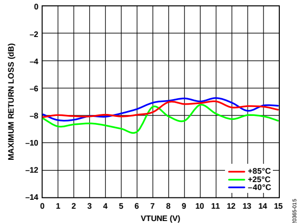
Figure 17. Maximum Return Loss in a 2 dB Bandwidth vs. VTUNE at Various Temperatures
