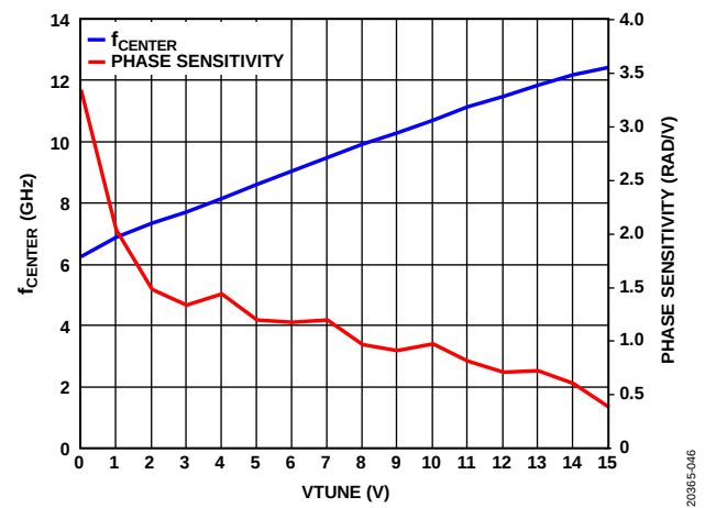
Figure 45. f_{\text{CENTER}} and Phase Sensitivity vs. VTUNE, Low Band
