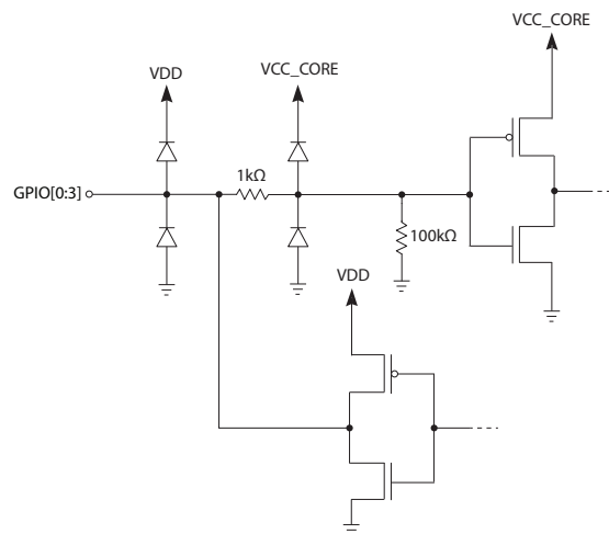
Figure 3-6: GPIO[0:3]
