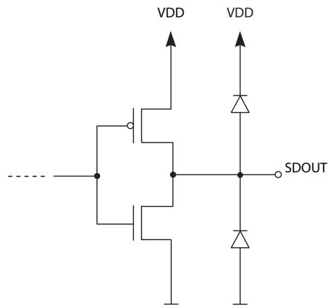
Figure 3-4: SDOUT
