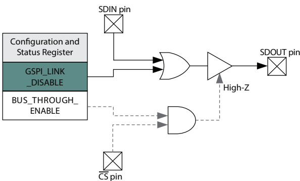
Figure 4-5: GSPI_LINK_DISABLE Operation
