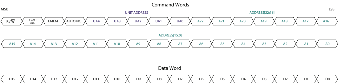
Figure 4-7: Command and Data Word Format
