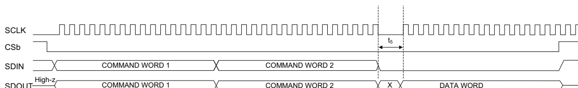
Figure 4-14: GSPI Read Timing—Single Read Access with Bus-through Operation
