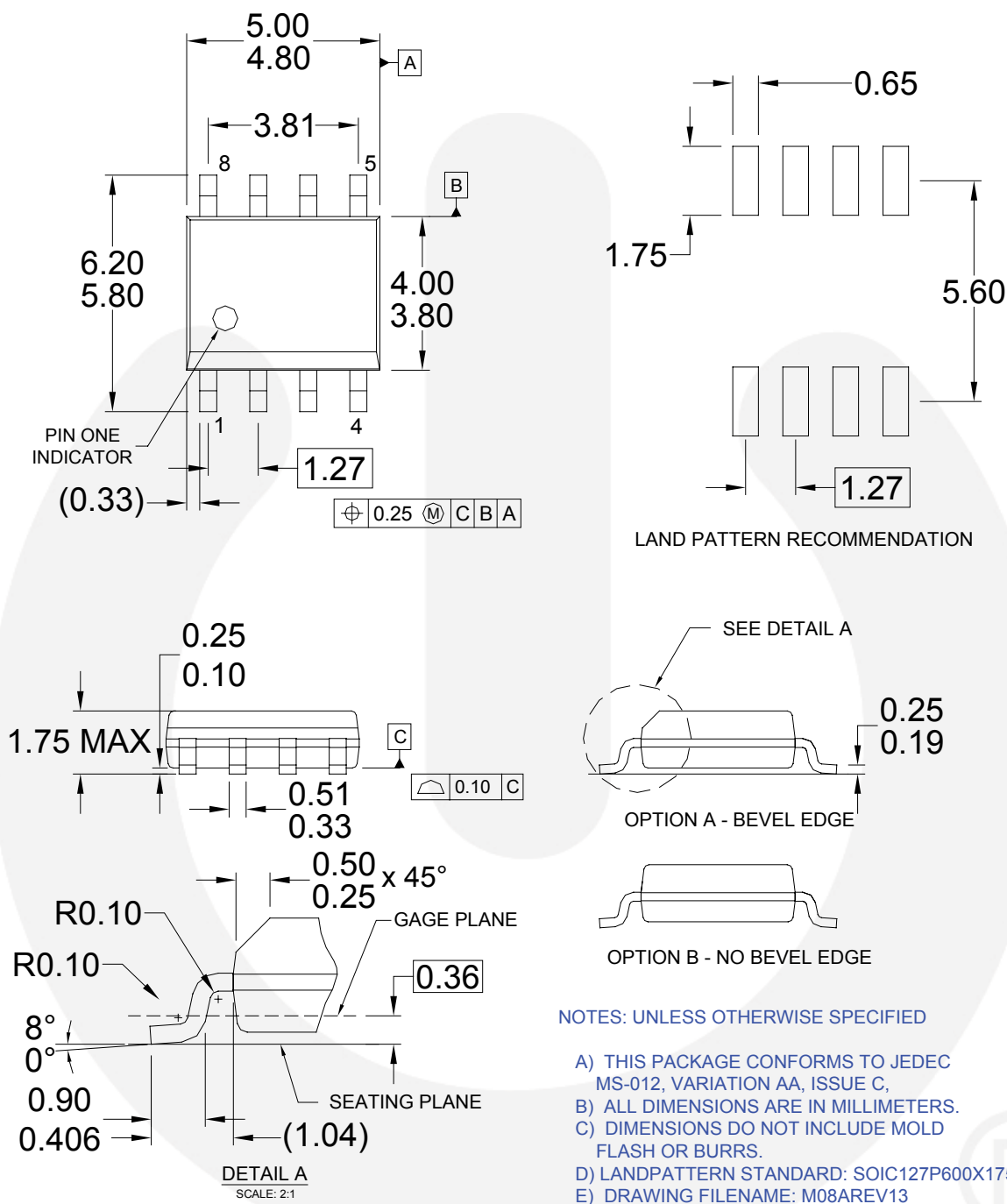
Figure 19. SOIC-8 Package
