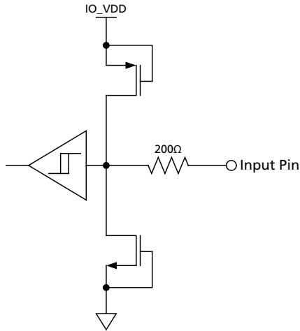
Figure 3-1: Digital Input Pin with Schmitt Trigger (20BIT/10BIT, \overline{CS\_TMS} , SW_EN, IOPROC_EN/ \overline{DIS} , JTAG/ \overline{HOST} , \overline{RC\_BYP} , \overline{RESET\_TRST} , SCLK_TCK, SDIN_TDI, SDO_EN/ \overline{DIS} , STANDBY, TIM_861)
