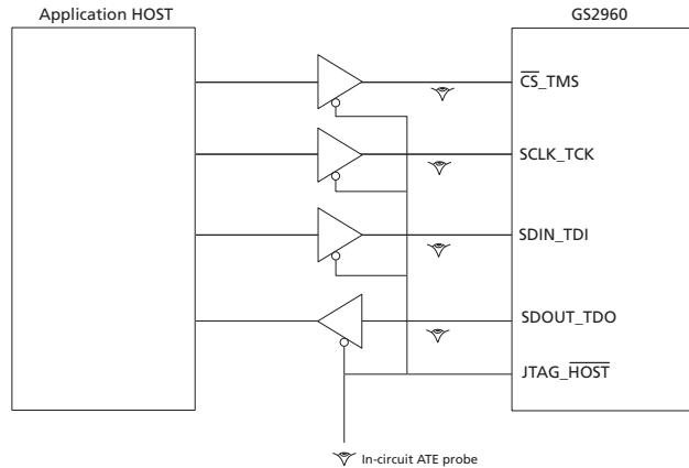
Figure 4-39: In-Circuit JTAG
