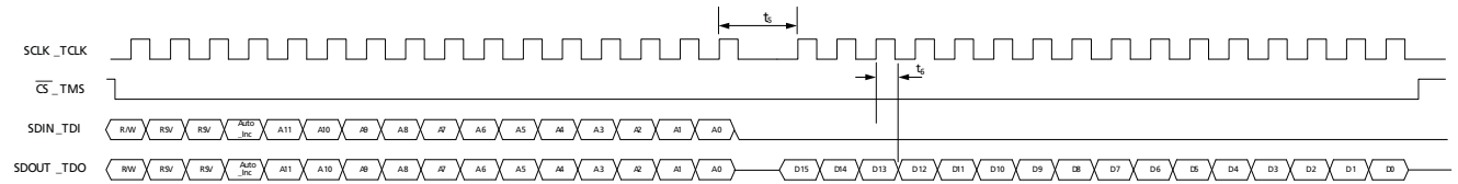
Figure 4-37: Read Mode
