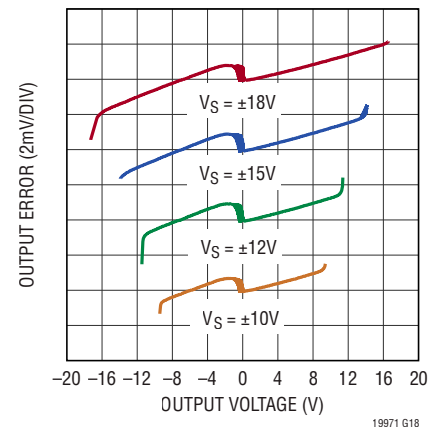
Typical Gain Error for R_L = 2\text{k}\Omega ( G = 10 ) (Curves Offset for Clarity)
