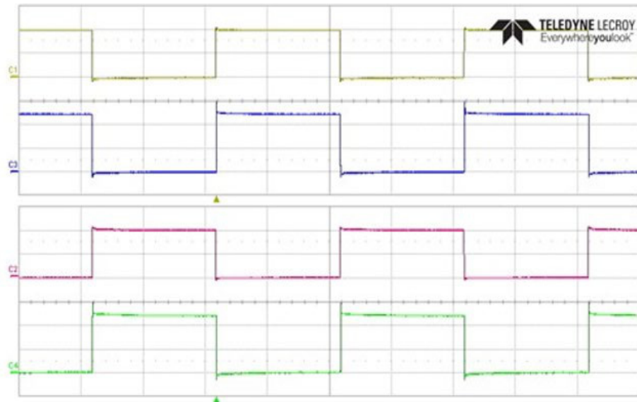
Figure 13. Experimental Waveforms if DT is Left Open
