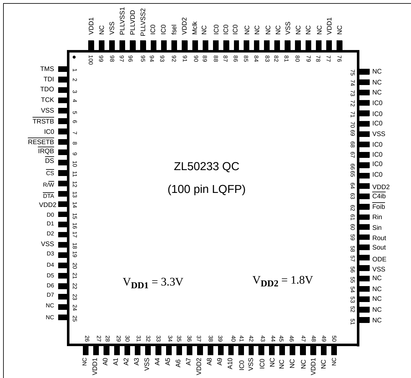
Figure 2 - 100 Pin LQFP
