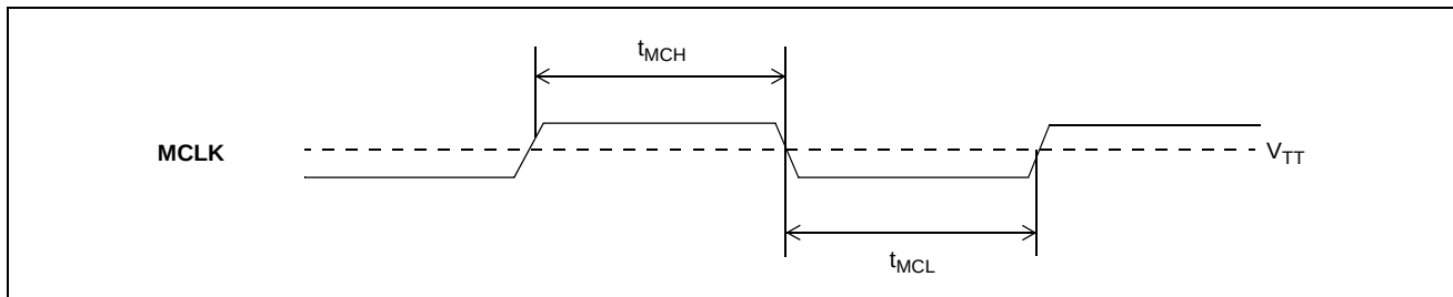
Figure 16 - Master Clock
