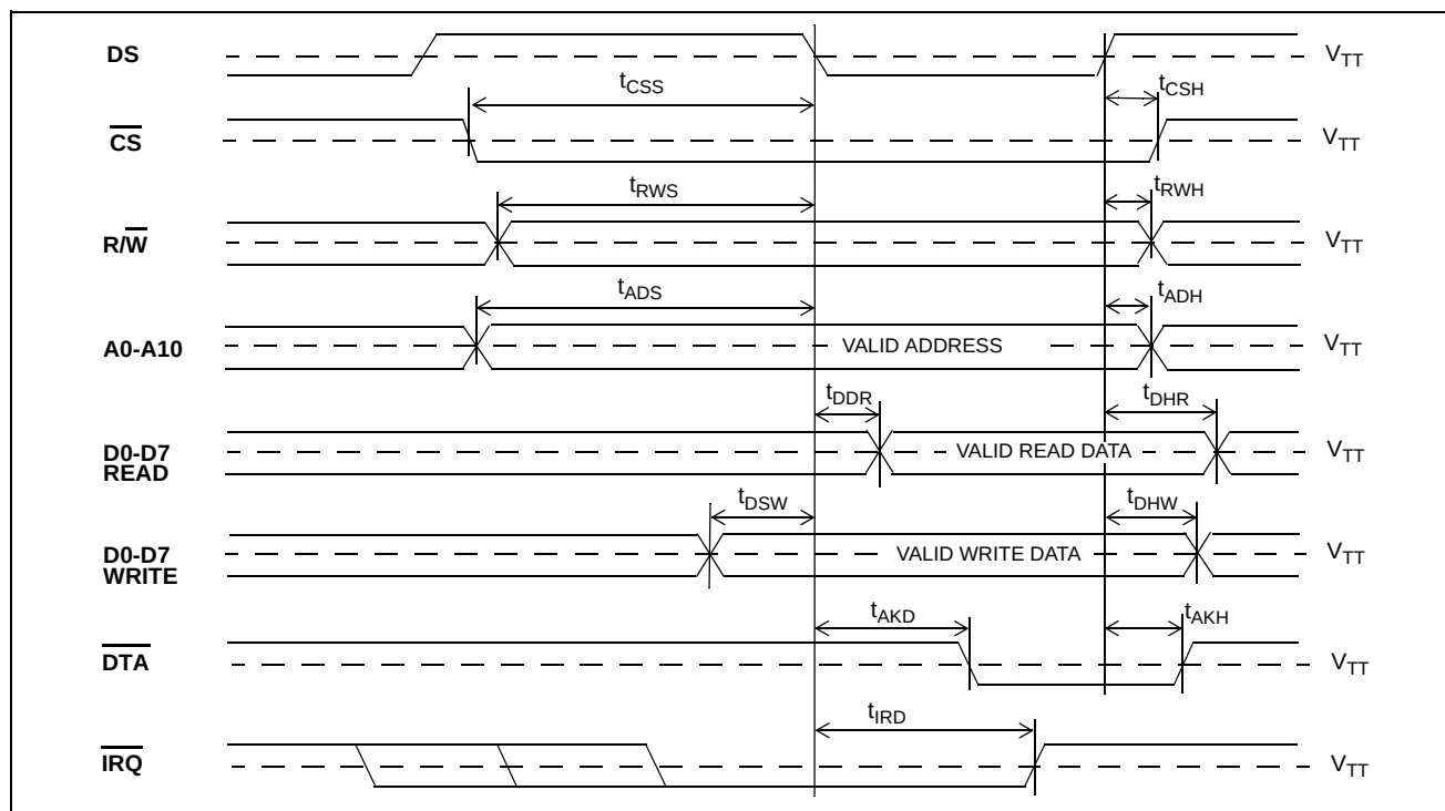
Figure 17 - Motorola Non-Multiplexed Bus Timing
