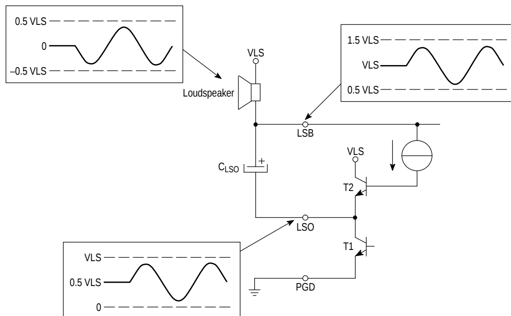
Figure 10. Loudspeaker Amplifier Output Power with External Supply
