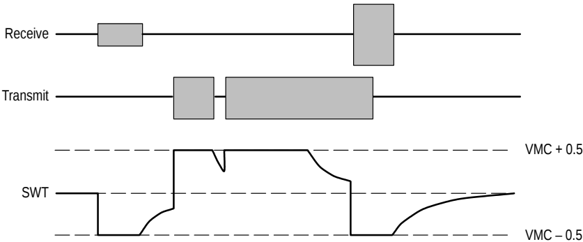
Figure 16. Switch-Over Behavior
