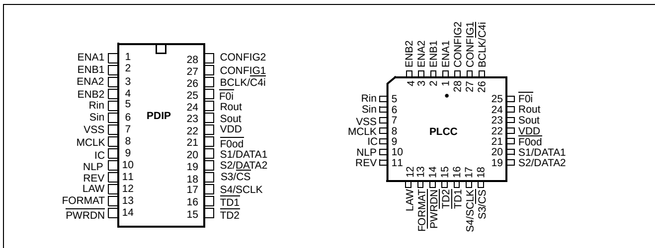
Figure 2 - Pin Connections
