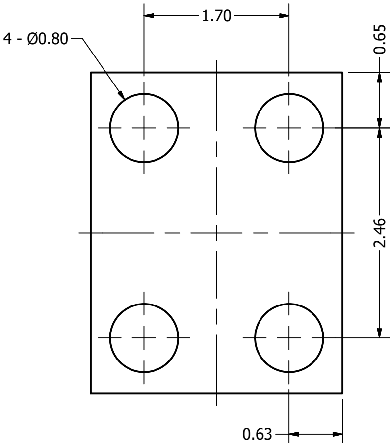
Bottom View (1)
