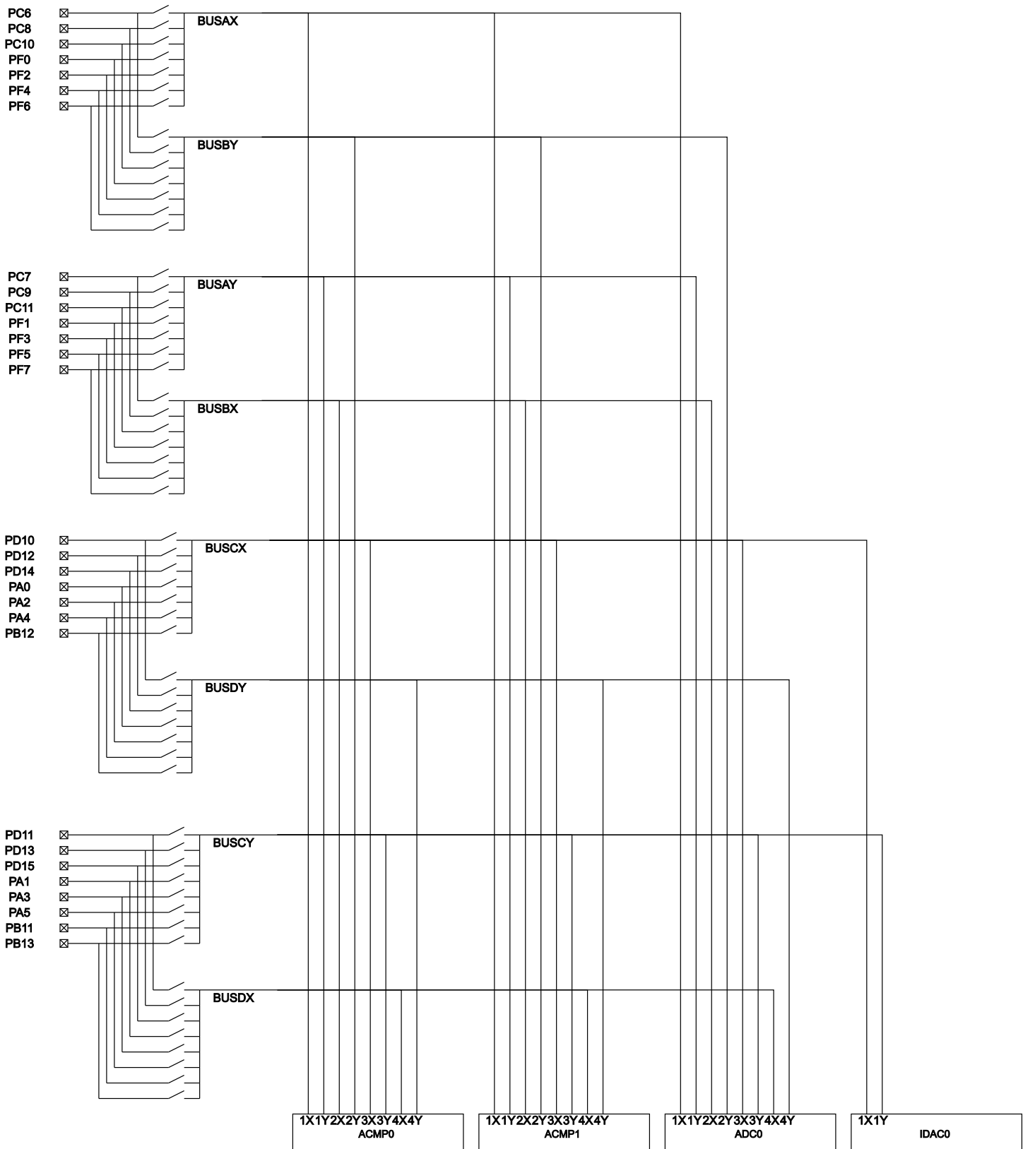
Figure 7.2. BGM121/BGM123 APORT
