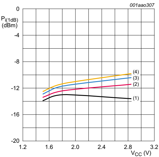
f = 1575 \text{ MHz} . (1) T_{\text{amb}} = -40 \text{ }^\circ\text{C} (2) T_{\text{amb}} = +25 \text{ }^\circ\text{C} (3) T_{\text{amb}} = +85 \text{ }^\circ\text{C} (4) T_{\text{amb}} = +125 \text{ }^\circ\text{C}
