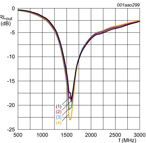
V_{\text{CC}} = 1.8 \text{ V} ; P_i = -45 \text{ dBm} . (1) T_{\text{amb}} = -40 \text{ }^{\circ}\text{C} (2) T_{\text{amb}} = +25 \text{ }^{\circ}\text{C} (3) T_{\text{amb}} = +85 \text{ }^{\circ}\text{C} (4) T_{\text{amb}} = +125 \text{ }^{\circ}\text{C}
