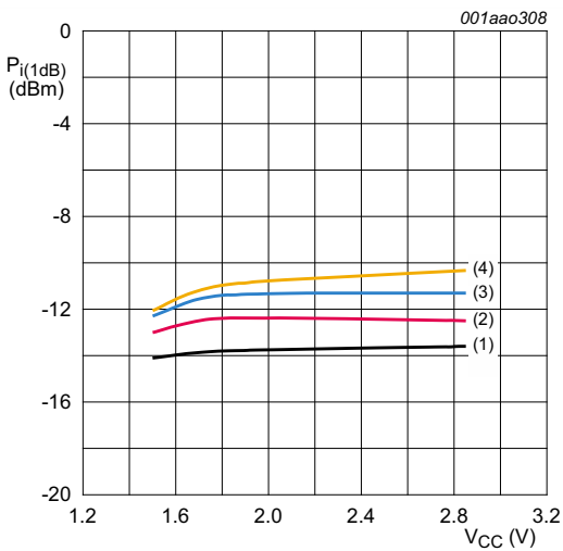
f = 850 \text{ MHz} . (1) T_{\text{amb}} = -40 \text{ }^\circ\text{C} (2) T_{\text{amb}} = +25 \text{ }^\circ\text{C} (3) T_{\text{amb}} = +85 \text{ }^\circ\text{C} (4) T_{\text{amb}} = +125 \text{ }^\circ\text{C}
