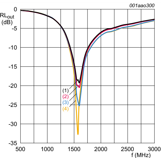
V_{\text{CC}} = 1.8 \text{ V} ; T_{\text{amb}} = 25 \text{ }^{\circ}\text{C} . (1) P_i = -45 \text{ dBm} (2) P_i = -30 \text{ dBm} (3) P_i = -20 \text{ dBm} (4) P_i = -15 \text{ dBm}
