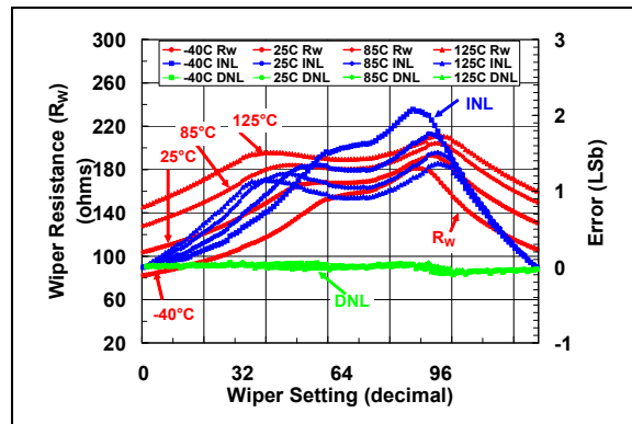
FIGURE 2-7: 5.0\text{ k}\Omega : Rheo Mode – R_W ( \Omega ), INL (LSb), DNL (LSb) vs. Wiper Setting and Temperature ( V_{DD} = 2.7\text{V} ). ( I_W = 450\mu\text{A} , B = V_{SS} ).
