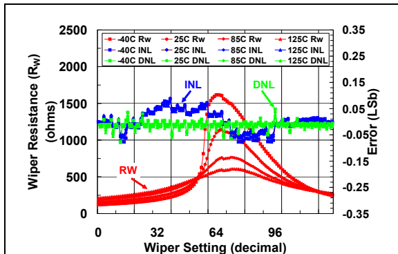
FIGURE 2-4: 5.0\text{ k}\Omega : Pot Mode – R_W ( \Omega ), INL (LSb), DNL (LSb) vs. Wiper Setting and Temperature ( V_{DD} = 2.7\text{V} ). ( A = V_{DD} , B = V_{SS} ).
