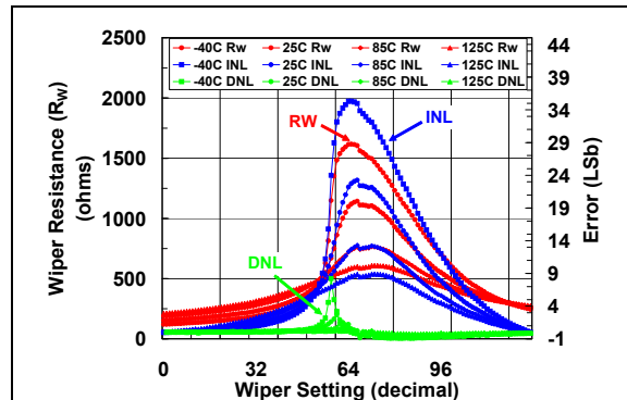
FIGURE 2-7: 5.0\text{ k}\Omega : Rheo Mode – R_W ( \Omega ), INL (LSb), DNL (LSb) vs. Wiper Setting and Temperature ( V_{DD} = 2.7\text{V} ). ( I_W = 450\mu\text{A} , B = V_{SS} ).
