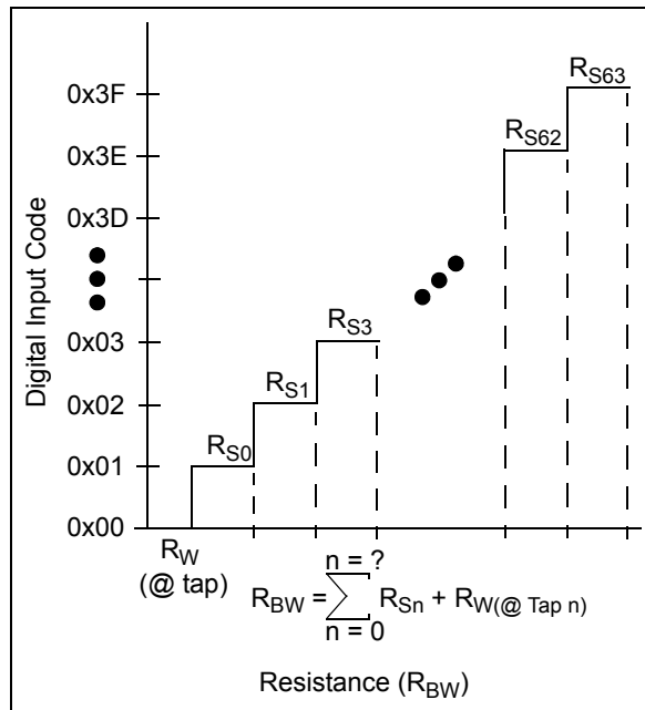
FIGURE 6-7: R_{BW}
