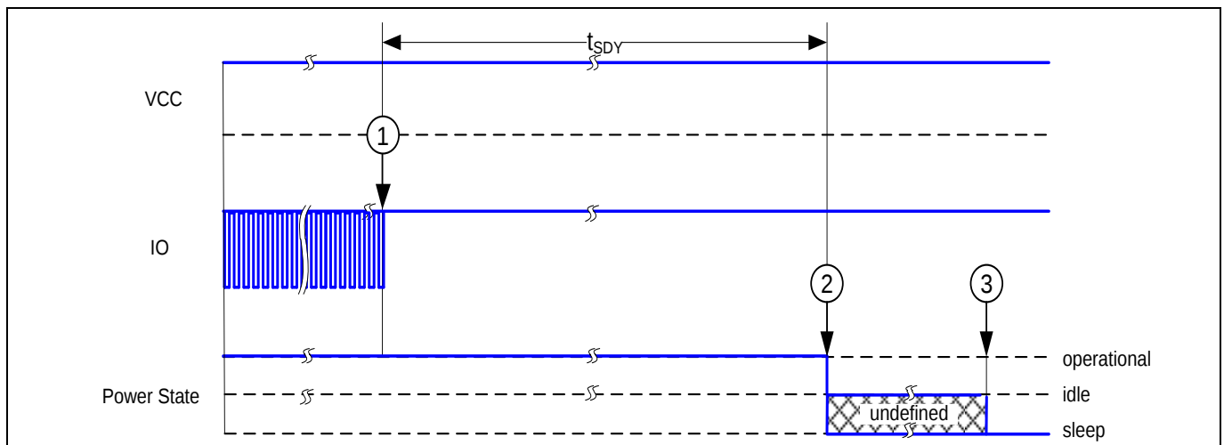
Figure 13 Go-to-Sleep Diagram
