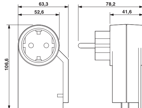
Dimensional drawing MNT-TV-SAT D
