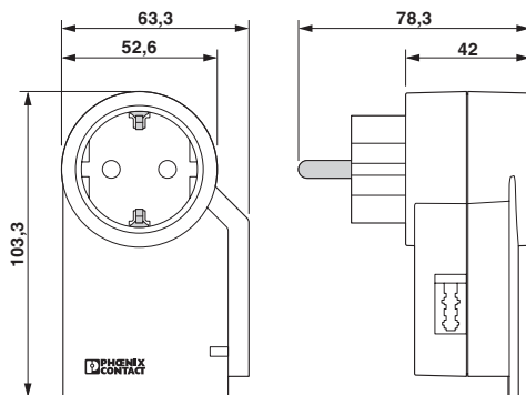
Dimensional drawing MNT-TAE D
