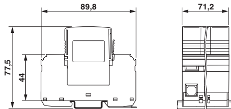
Dimensional drawing VAL-MS-T1/T2 335/12.5/3+1
