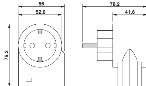
Dimensional drawing MNT-1 D
