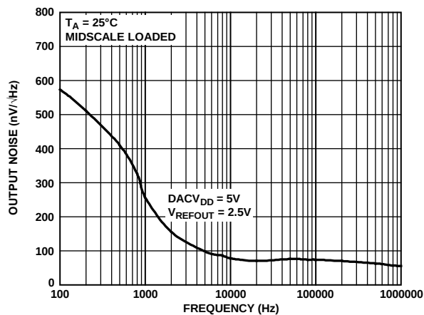
Figure 21. DAC Noise Spectral Density, Internal Reference
