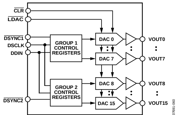
Figure 60. DAC Serial Interface Configuration
