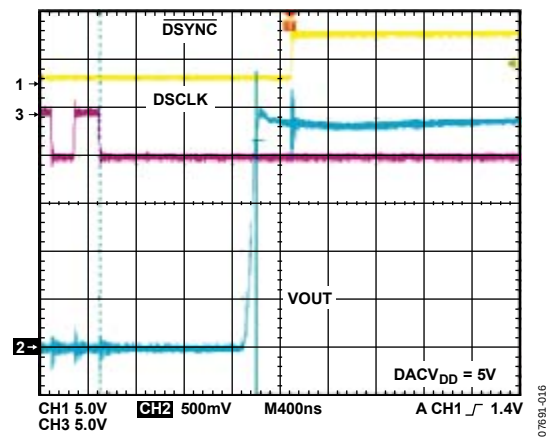
Figure 16. DAC Exiting Power-Down to Midscale
