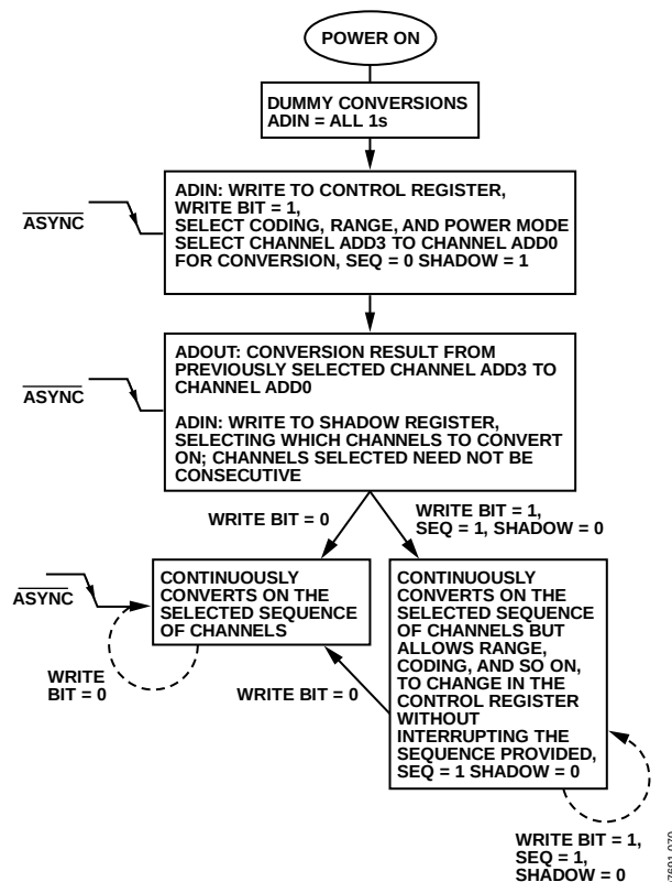
Figure 70. Continuous Conversions
