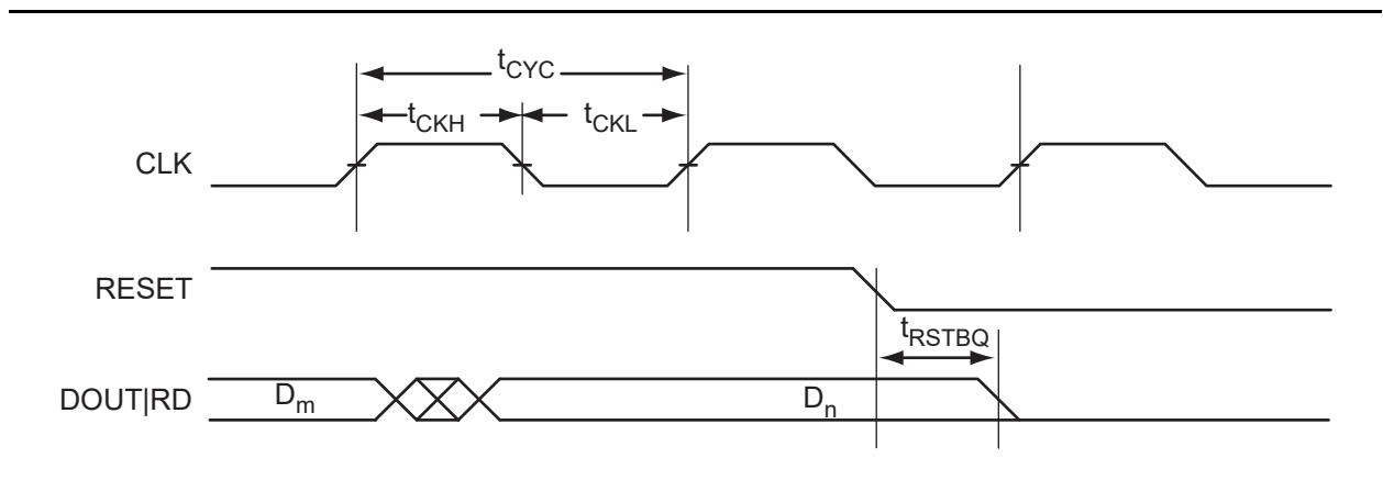
Figure 2-28 • RAM Reset
