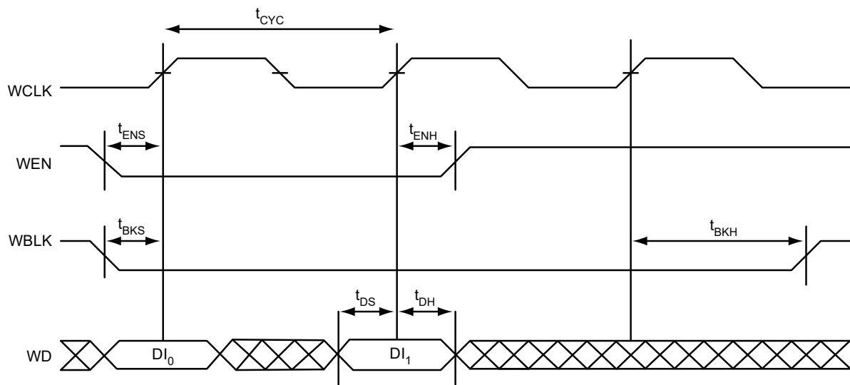
Figure 2-31 • FIFO Write
