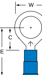
MNG14-38R Stud Size 3/8 Wire Range 16-14
