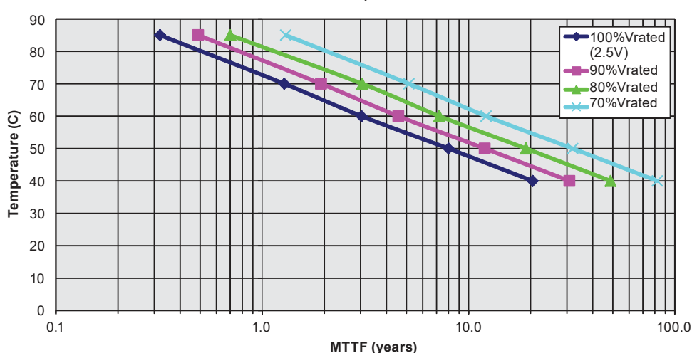
Expected Lifetime at Various Voltages SCC series, 2.5V Rated
