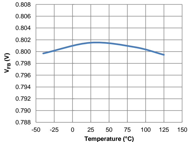
Figure 10. Feedback Voltage vs. Temperature
