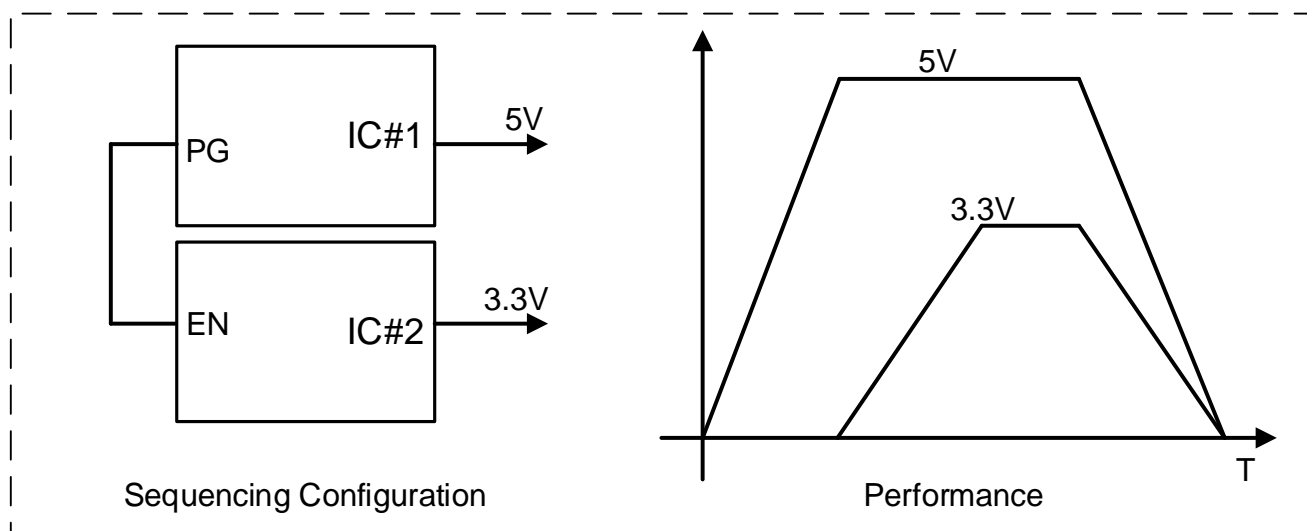
Figure 39. Sequencing Configuration
