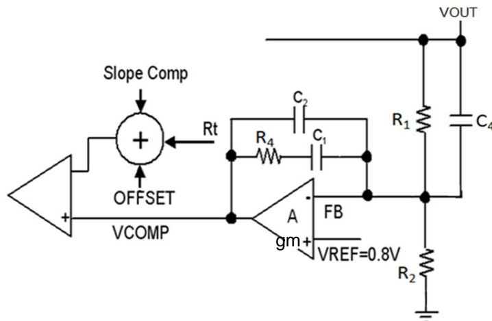
Figure 46. Type 2 Compensator
