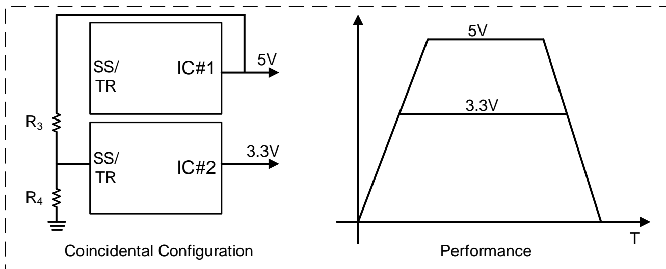
Figure 38. Coincidental Configuration
