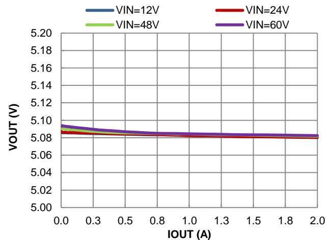
Figure 16. Load Regulation
