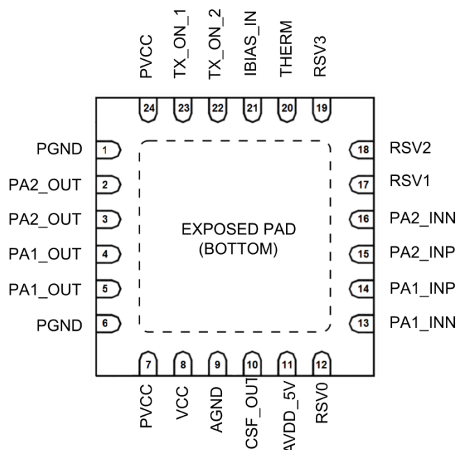
Figure 3. Pin connections
