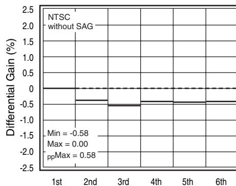
Figure 6. Differential Gain
