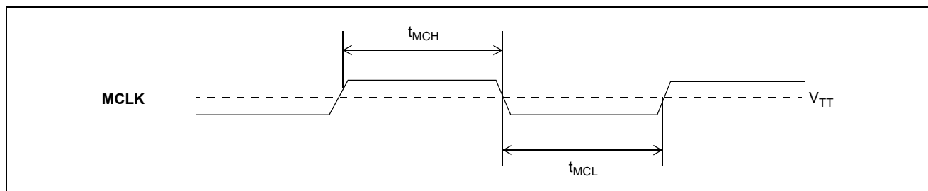
Figure 17 - Master Clock
