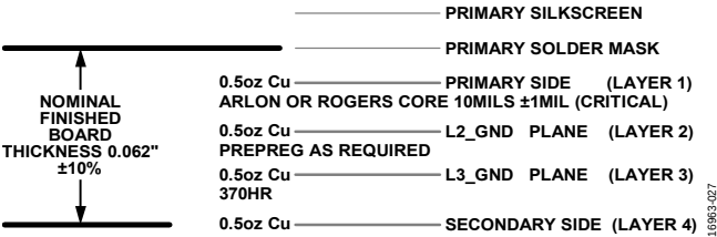
Figure 27. 4-Layer Stackup
