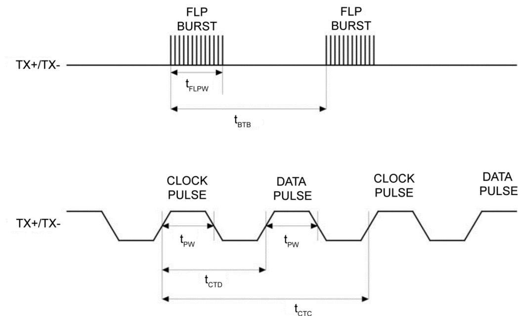
Figure 17. Auto-Negotiation Fast Link Pulse (FLP) Timing
