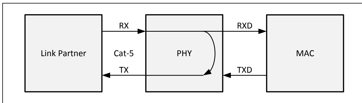
FIGURE 9-1: FAR-END LOOPBACK DIAGRAM
