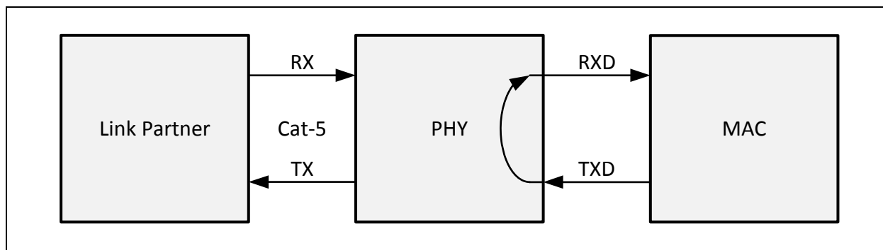
FIGURE 9-2: NEAR-END LOOPBACK DIAGRAM
