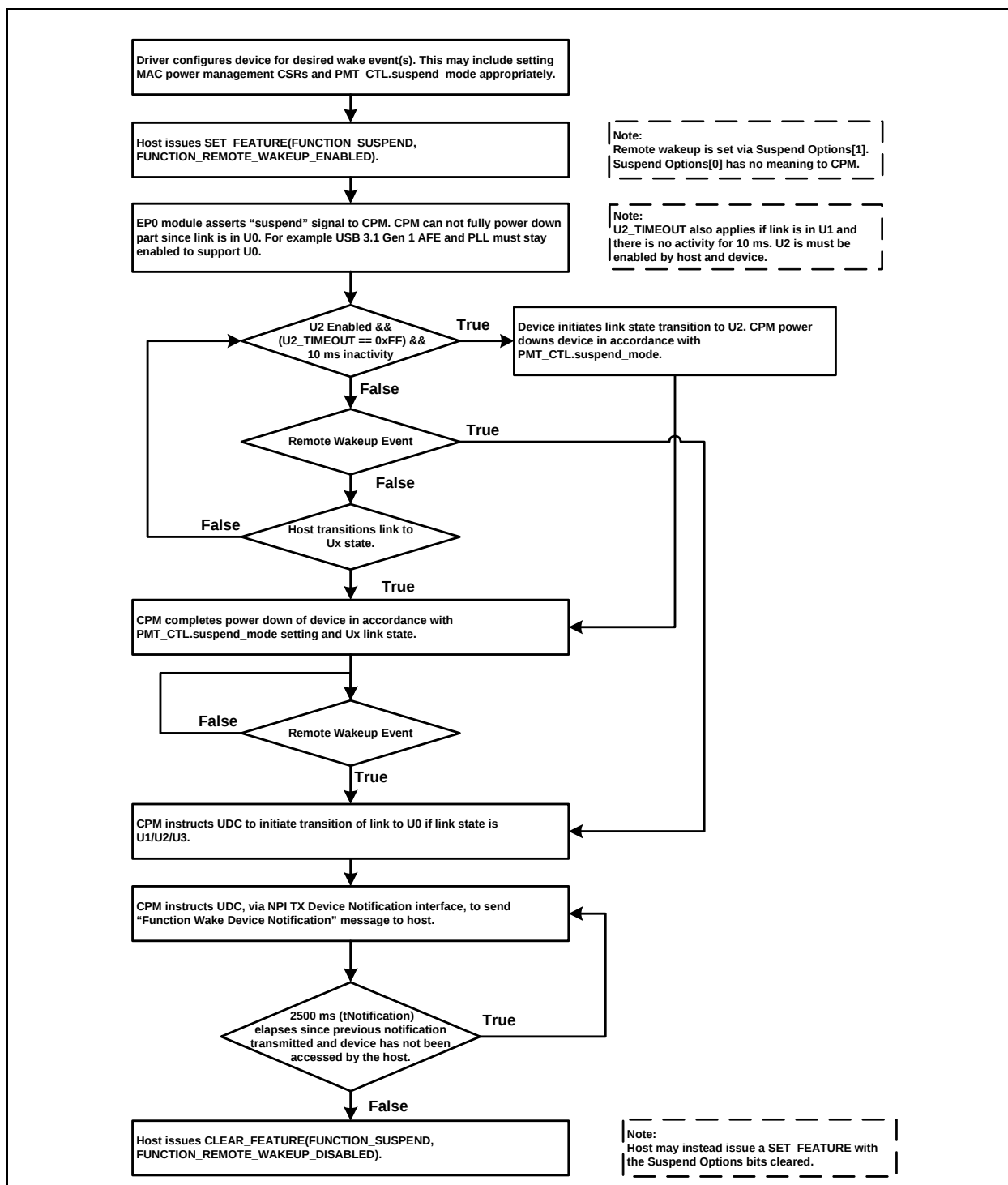
FIGURE 5-2: FUNCTION SUSPEND
