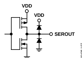
Figure 8. SEROUT Pin Interface
