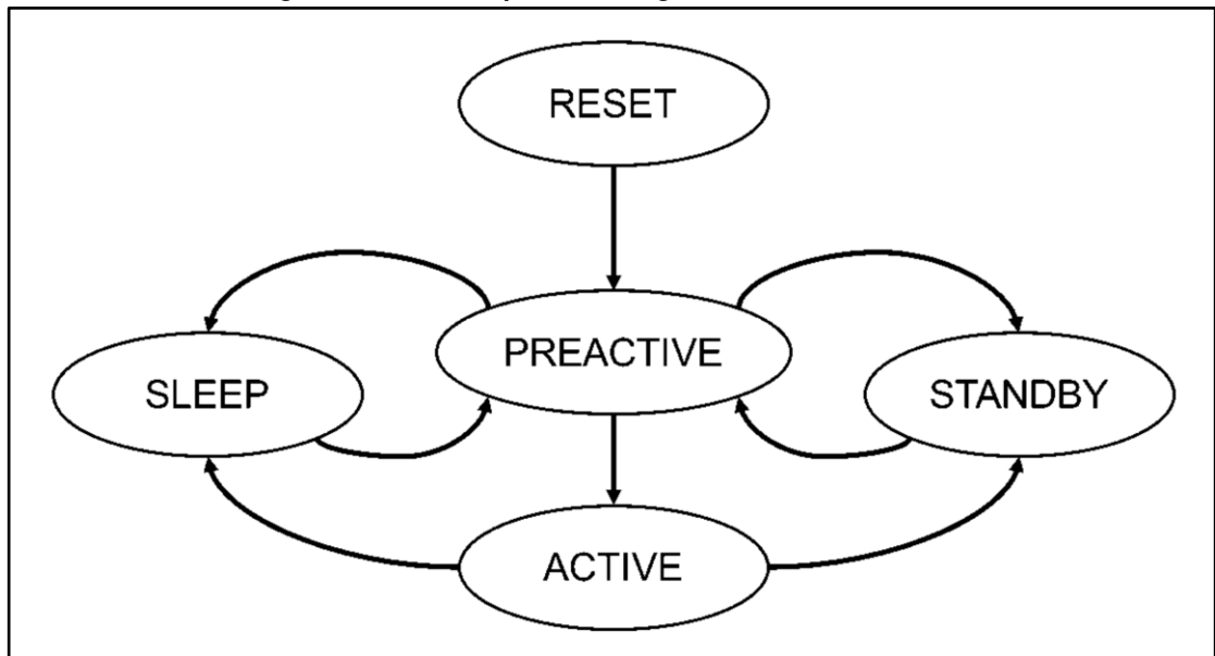
Figure 5: BlueNRG-1 power management state machine
