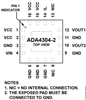
Figure 4. Pin Configuration
