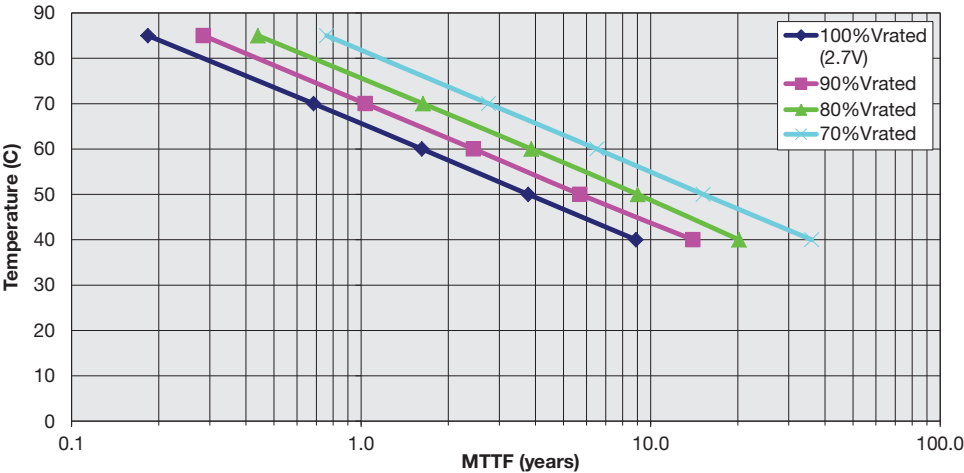
Expected Lifetime at Various Voltages SCM series 2.7V Rated
