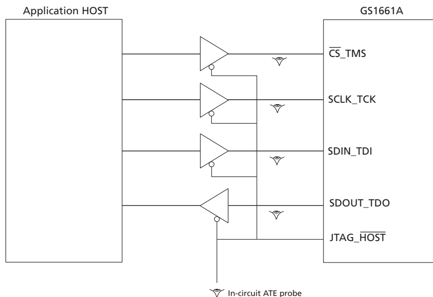
Figure 4-33: In-Circuit JTAG
