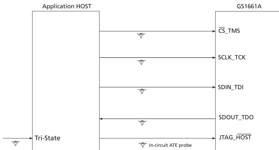
Figure 4-34: System JTAG
