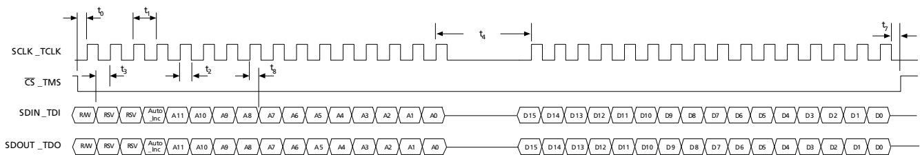
Figure 4-30: Write Mode
