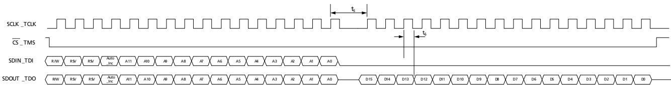
Figure 4-31: Read Mode
