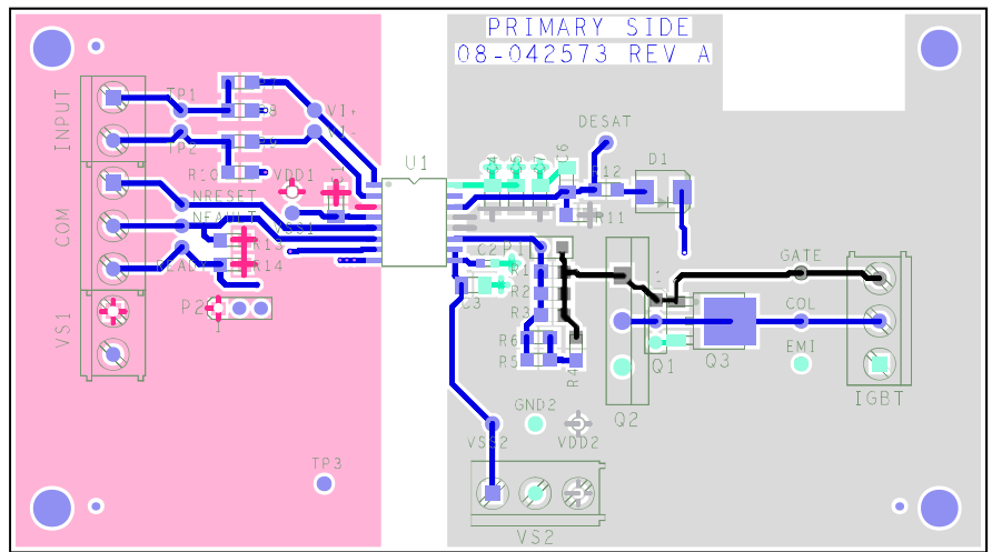
Figure 4. EVAL-ADuM4136EBZ Evaluation Board Top Layer
