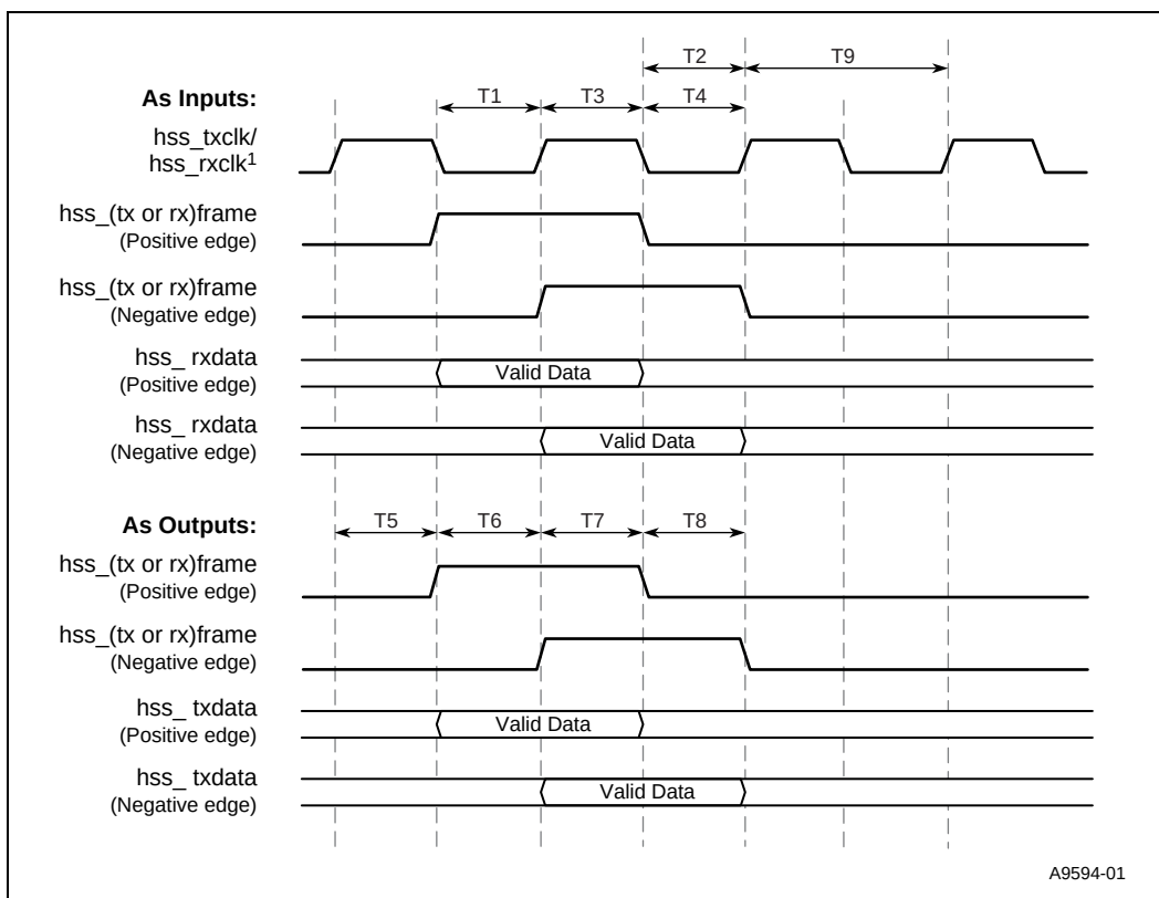
Figure 42. High-Speed, Serial Timings
