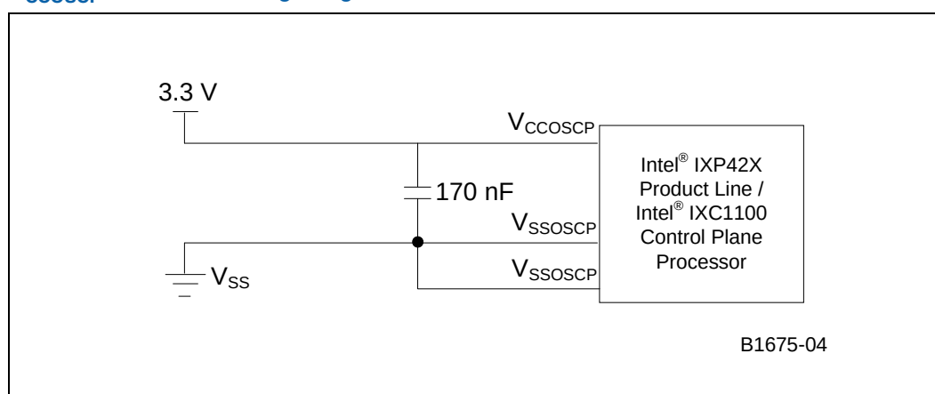
Figure 11. V_{CCOSC} Power Filtering Diagram
