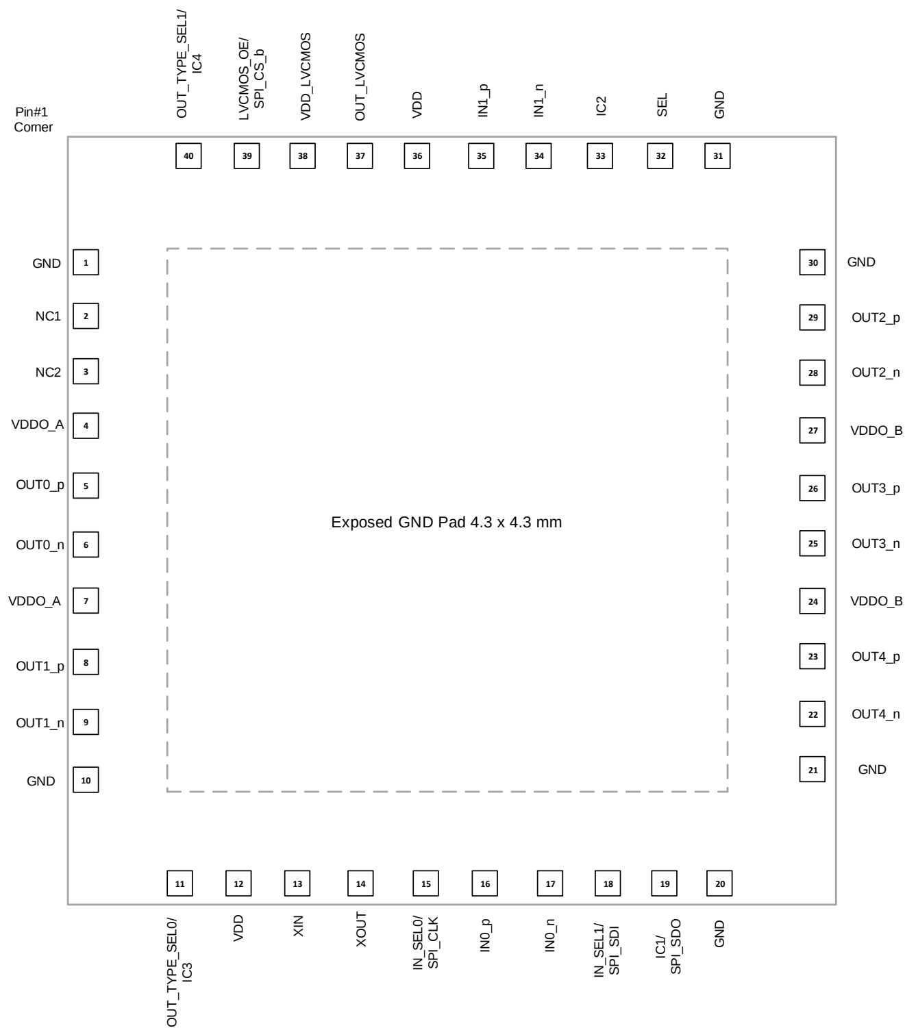
Figure 2. Pin Diagram
