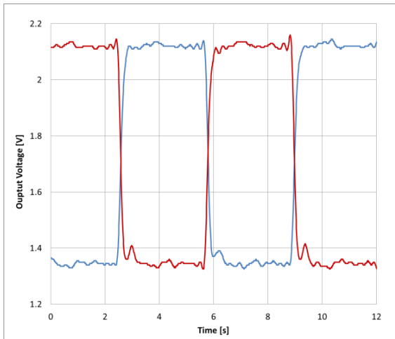
Figure 22. 156.25MHz LVPECL
