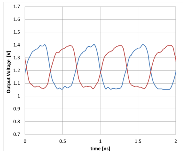
Figure 25. 1.5GHz LVDS
