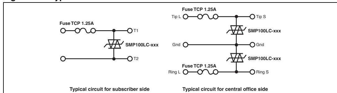
Figure 11. Typical circuits
