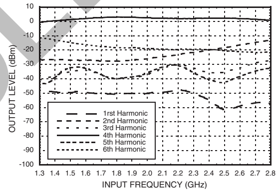
Spurious Output vs. Fin Pin = +5 dBm, T = 25 °C [1]
