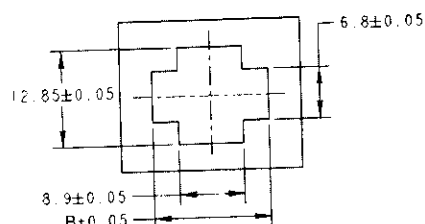
Panel Layout Panel thickness:1.0~2.0
