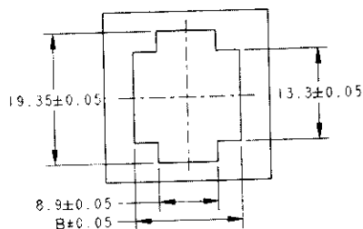
Panel Layout Panel thickness:1.0~2.0
