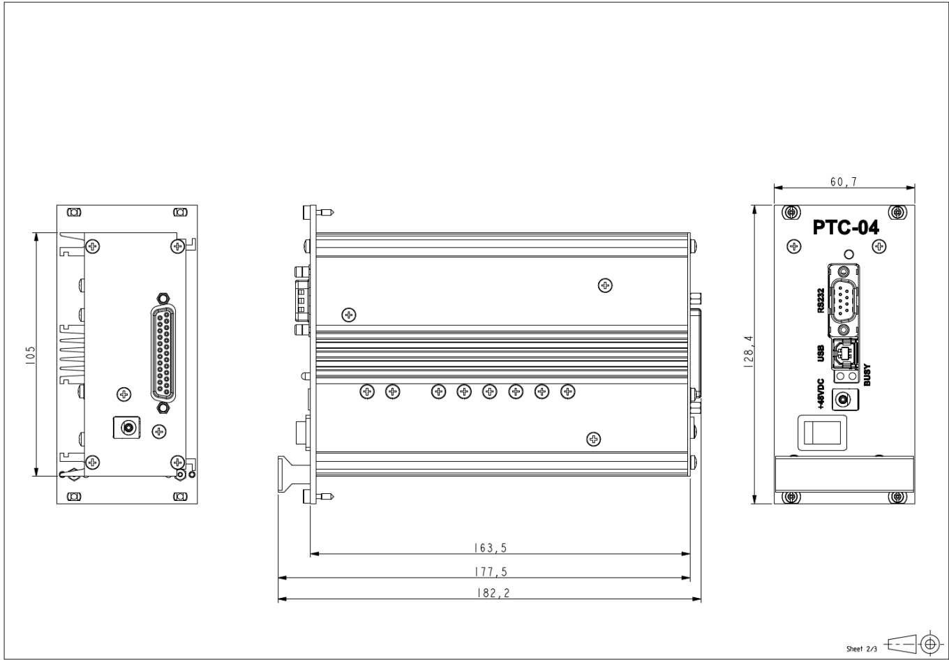
Figure 21-1: Mechanical Outlines
