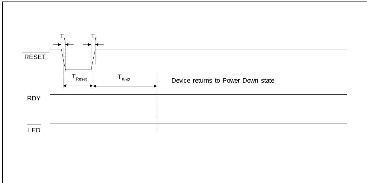
Figure 12.6: Reset Operation
