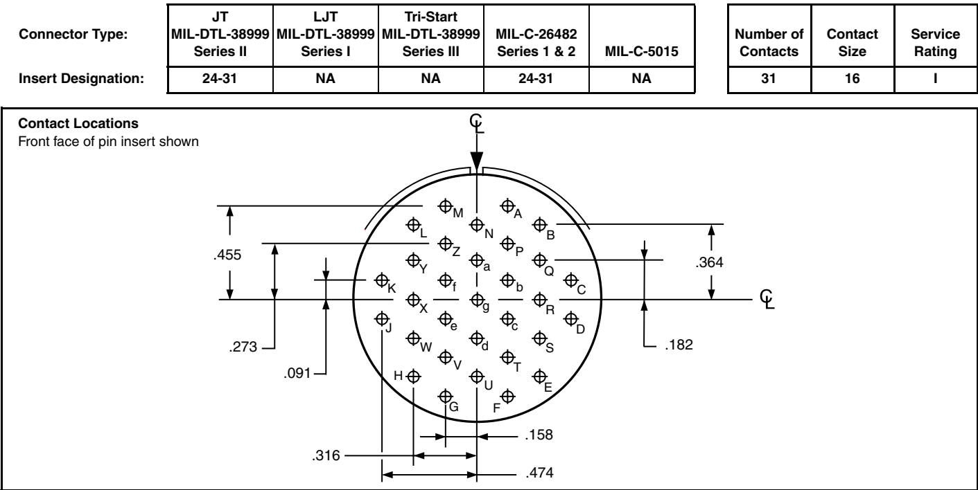
Insert Arrangement #24-31 / 25-31
