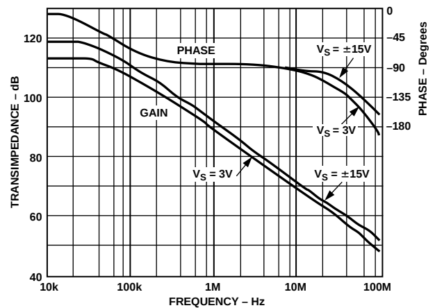
Figure 19. Open-Loop Transimpedance vs. Frequency (Relative to 1 \Omega )
