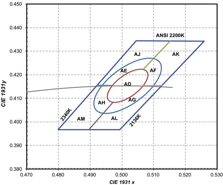
Figure 8a. 1/9 th color bin structure for LUXEON 2835E and LUXEON 2835C 2200K at test current and binning temperatures of T j =25°C and T j =85°C.
