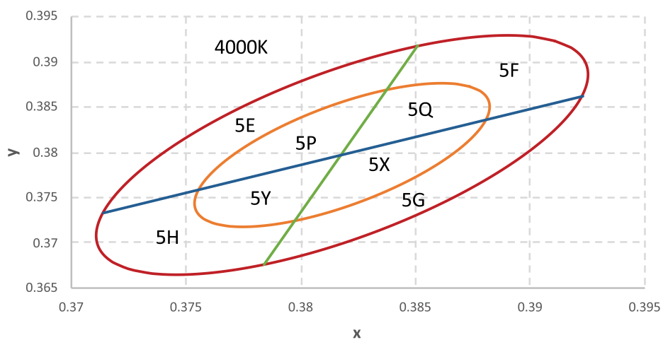
Figure 8I. 1/8 th color bin structure for LUXEON 2835 HE 4000K at test current and binning temperature of T_j=25^{\circ}\text{C} .
