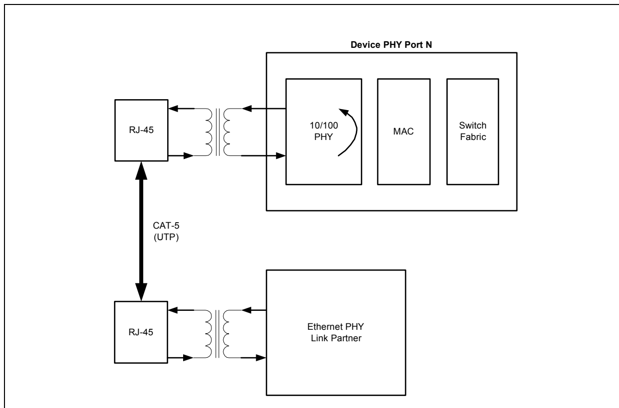
FIGURE 4-2: REMOTE PHY LOOPBACK
