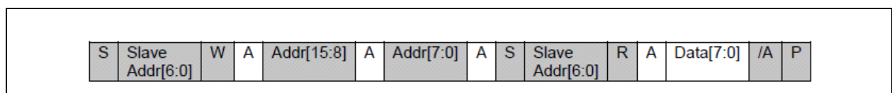
FIGURE 4-14: SINGLE BYTE REGISTER READ
