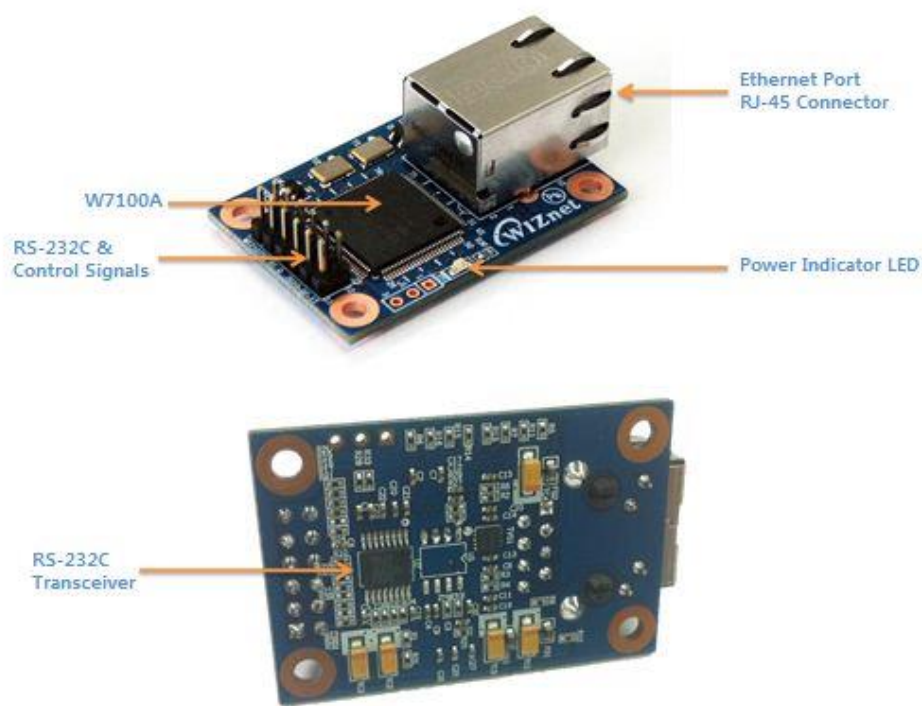
Figure 1. WIZ107SR Interface
