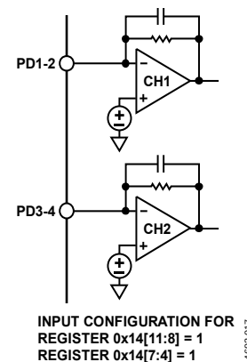
Figure 23. Current Summation—Two Photodiodes Summed into One Current
