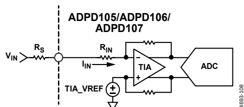
Figure 52. Using the ADPD105/ADPD106/ADPD107 Inputs with Voltage Sources
