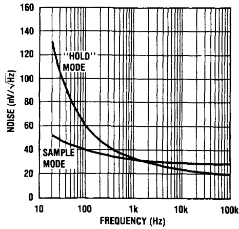
Output Noise
