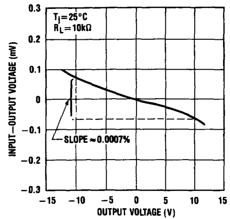
Gain Error
